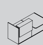
TRA36L 2056 / 1120 / 1159 81" / 44 1/8" / 45 5/8" TRA36P 2056 / 1120 / 1159 81" / 44 1/8" / 45 5/8" TRA37L 2256 / 1120 / 1159 88 7/8" / 44 1/8" / 45 5/8" TRA37P 2256 / 1120 / 1159 88 7/8" / 44 1/8" / 45 5/8" TRA38L 2456 / 1120 / 1159 96 3/4" / 44 1/8" / 45 5/8" TRA38P 2456 / 1120 / 1159 96 3/4" / 44 1/8" / 45 5/8"
