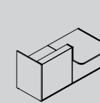
TRA136L 2056 / 1120 / 1159 81" / 44 1/8" / 45 5/8" TRA136P 2056 / 1120 / 1159 81" / 44 1/8" / 45 5/8" TRA137L 2256 / 1120 / 1159 88 7/8" / 44 1/8" / 45 5/8" TRA137P 2256 / 1120 / 1159 88 7/8" / 44 1/8" / 45 5/8" TRA138L 2456 / 1120 / 1159 96 3/4" / 44 1/8" / 45 5/8" TRA138P 2456 / 1120 / 1159 96 3/4" / 44 1/8" / 45 5/8"
